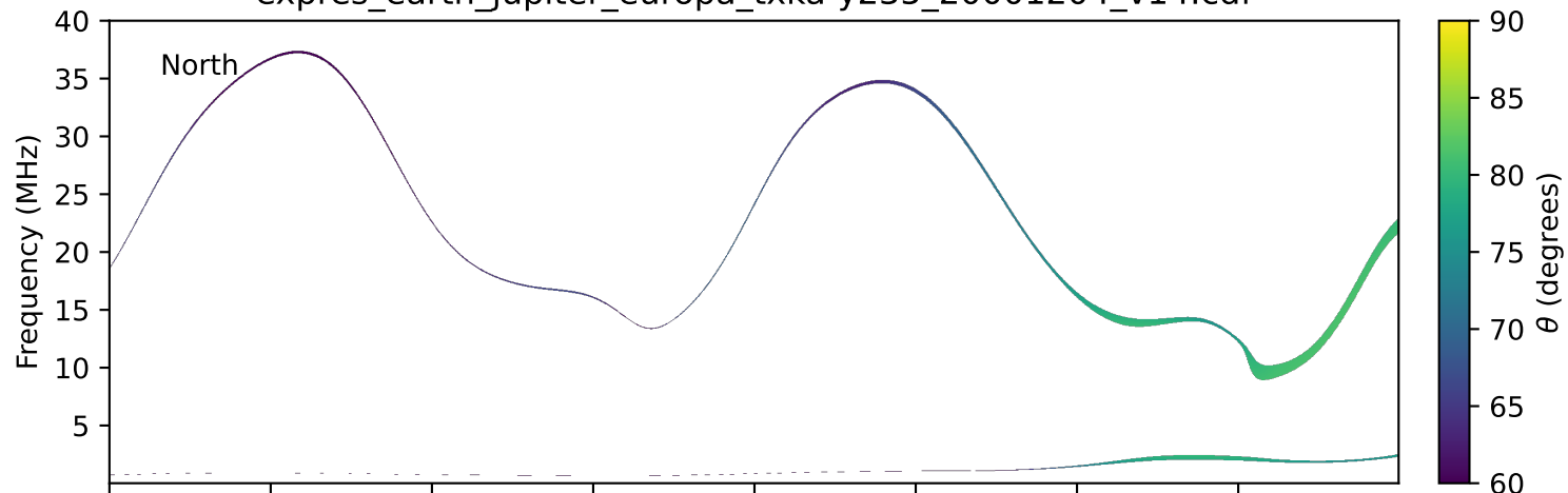
expres_earth_jupiter_europa_txka-y235_20001204_v14.cdf
