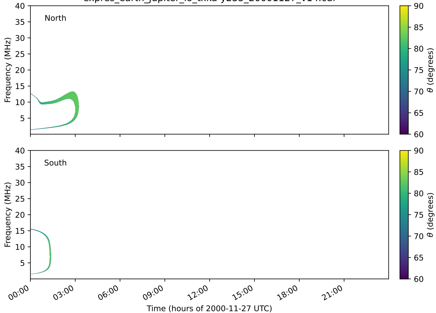
expres_earth_jupiter_io_txka-y235_20001127_v14.cdf
