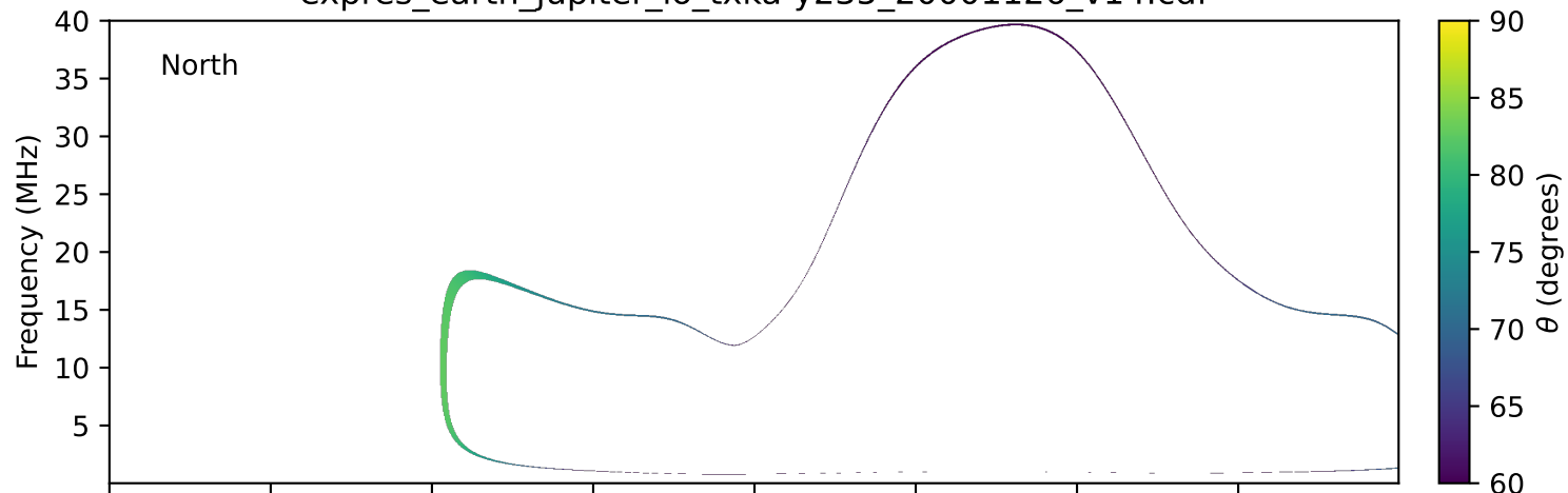
expres_earth_jupiter_io_txka-y235_20001126_v14.cdf
