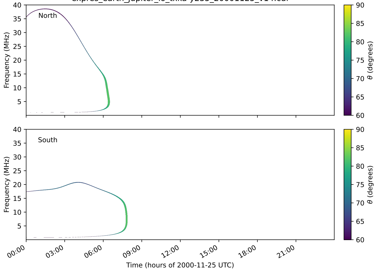
expres_earth_jupiter_io_txka-y235_20001125_v14.cdf
