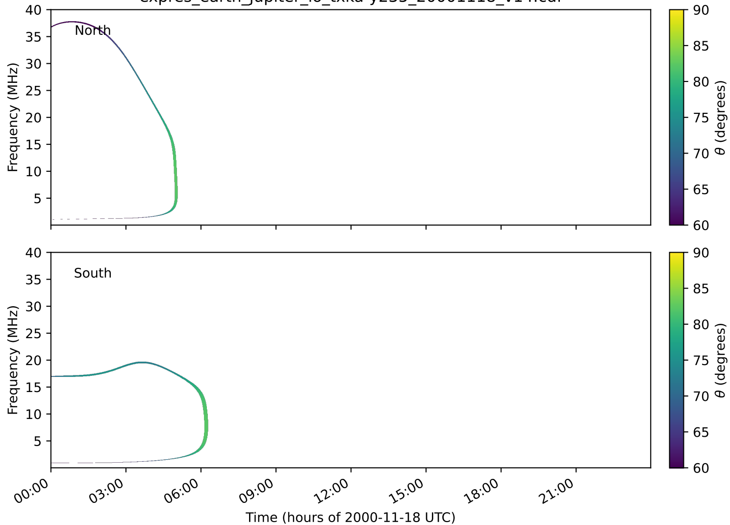
expres_earth_jupiter_io_txka-y235_20001118_v14.cdf
