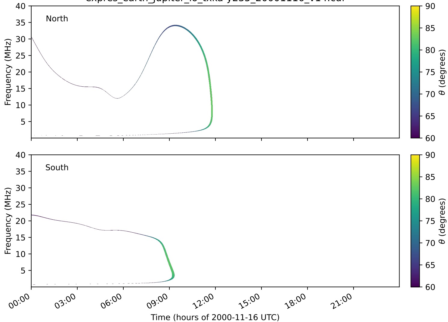
expres_earth_jupiter_io_txka-y235_20001116_v14.cdf
