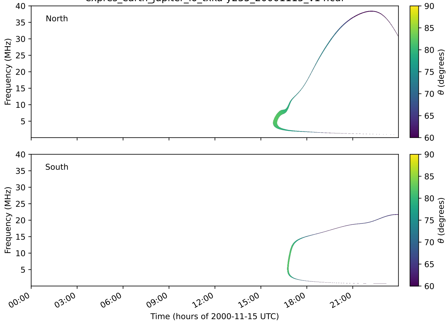
expres_earth_jupiter_io_txka-y235_20001115_v14.cdf
