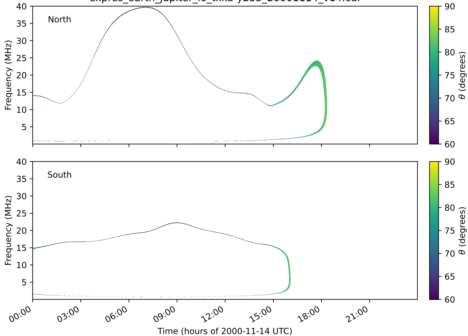
expres_earth_jupiter_io_txka-y235_20001114_v14.cdf
