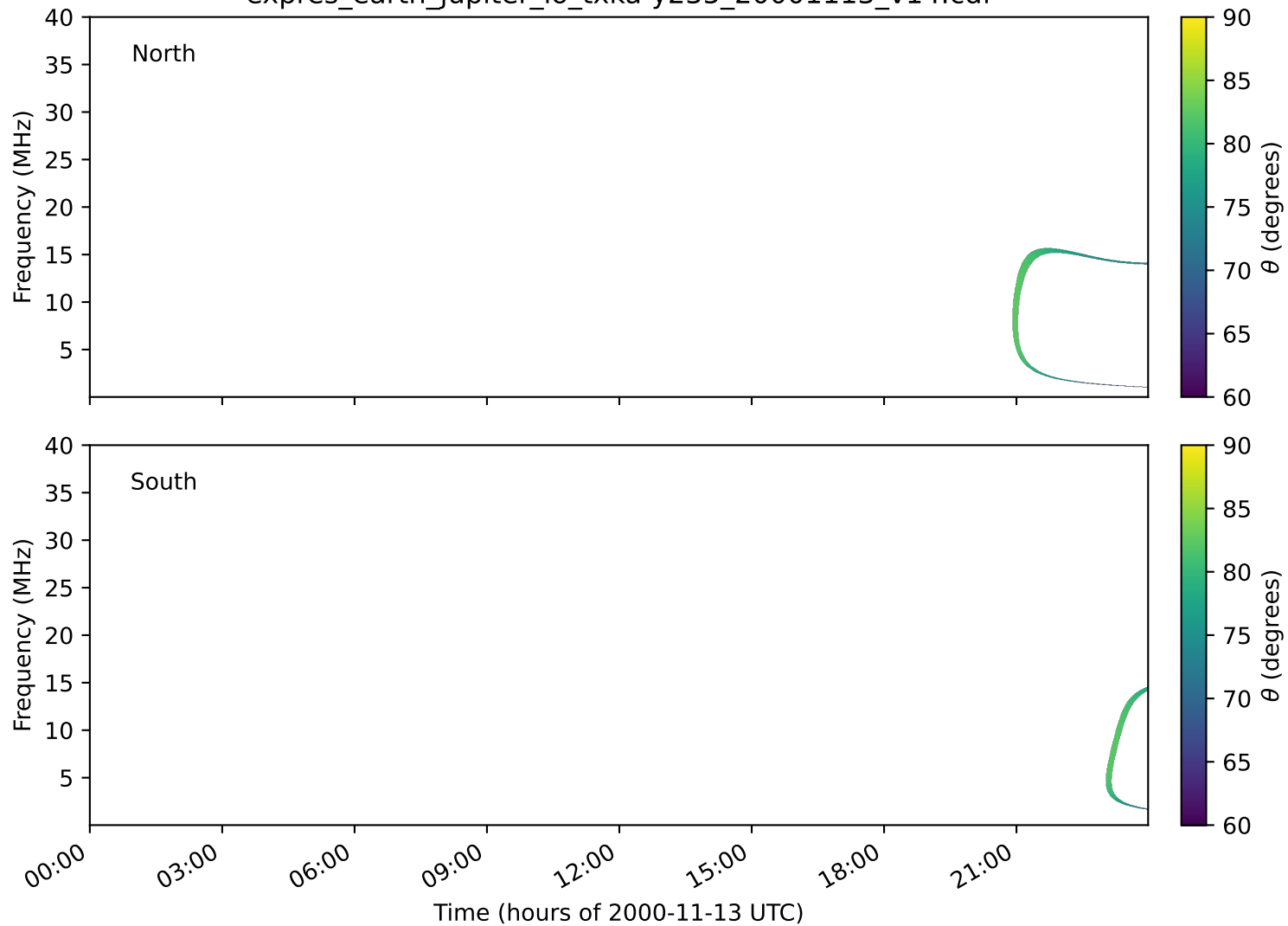
expres_earth_jupiter_io_txka-y235_20001113_v14.cdf
