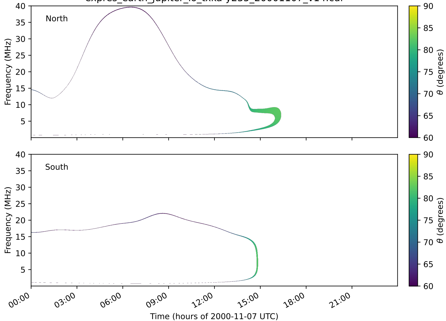
expres_earth_jupiter_io_txka-y235_20001107_v14.cdf
