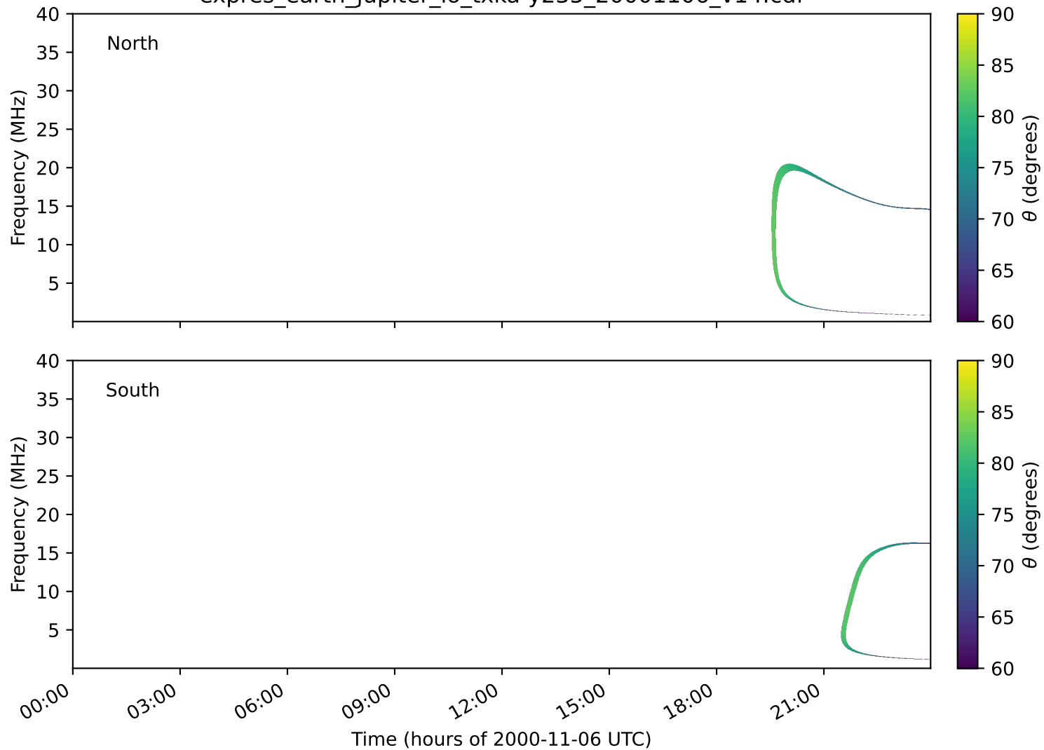
expres_earth_jupiter_io_txka-y235_20001106_v14.cdf
