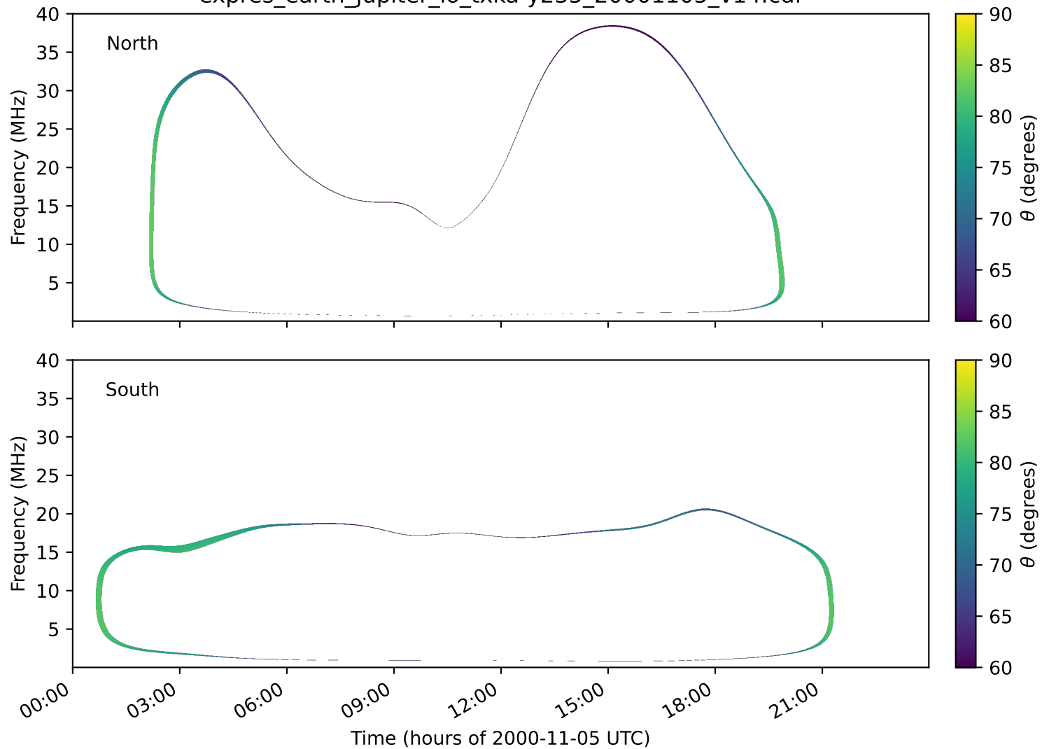
expres_earth_jupiter_io_txka-y235_20001105_v14.cdf
