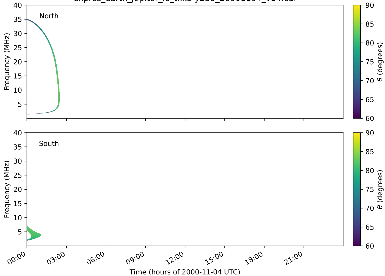
expres_earth_jupiter_io_txka-y235_20001104_v14.cdf
