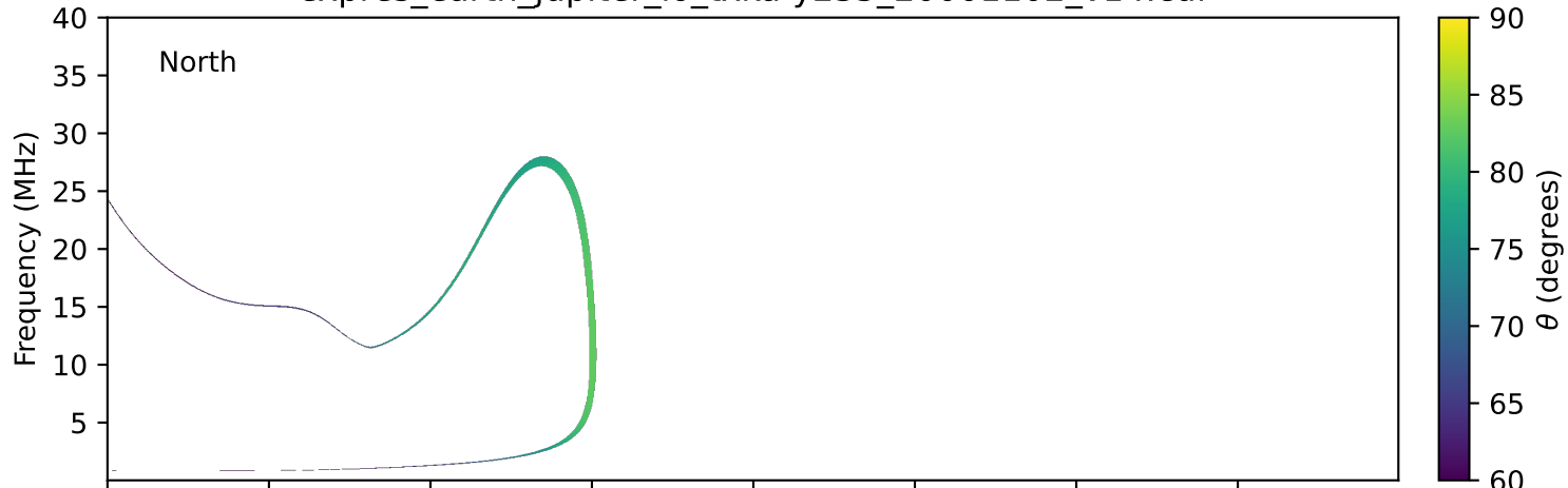
expres_earth_jupiter_io_txka-y235_20001102_v14.cdf
