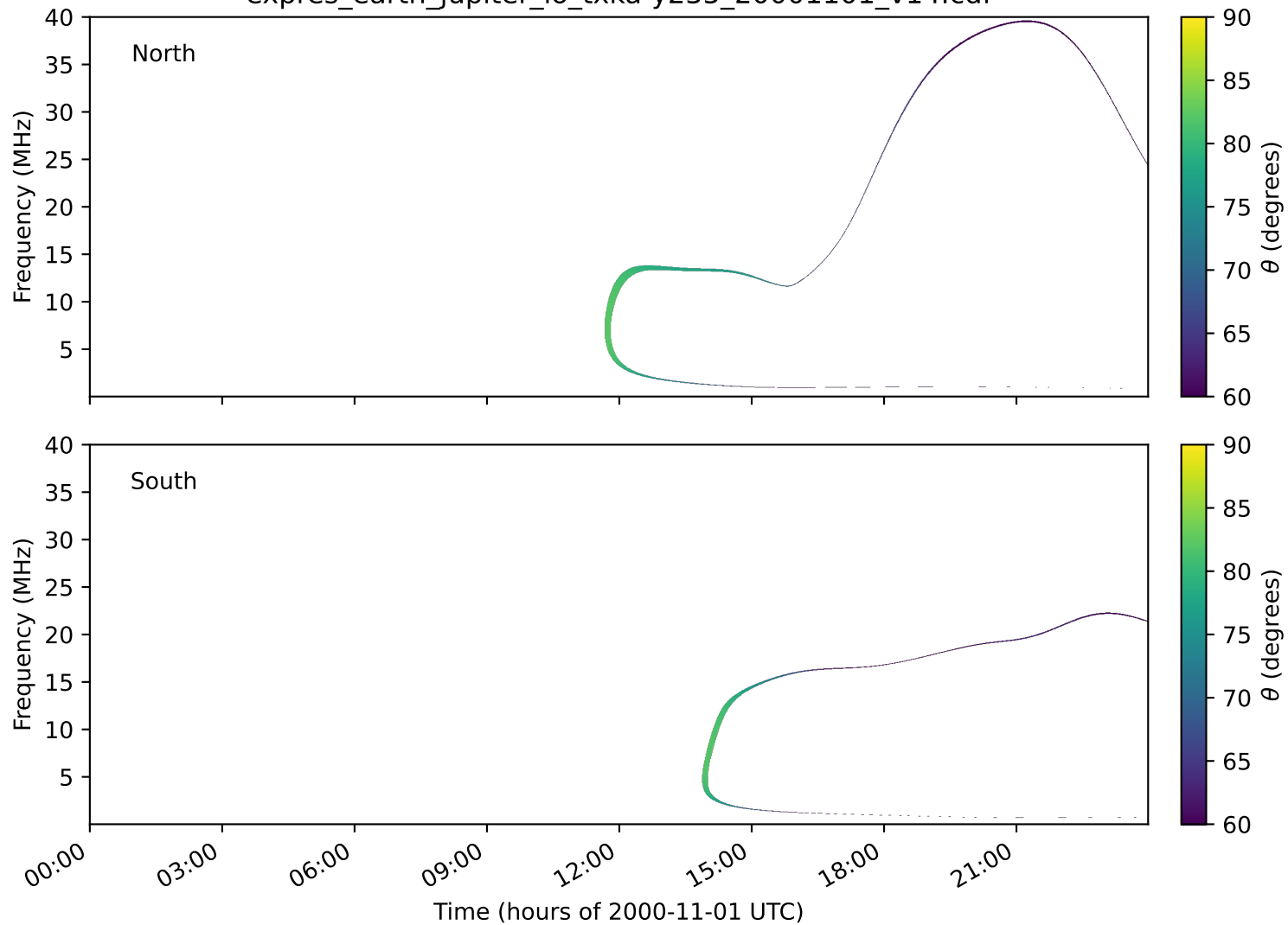
expres_earth_jupiter_io_txka-y235_20001101_v14.cdf
