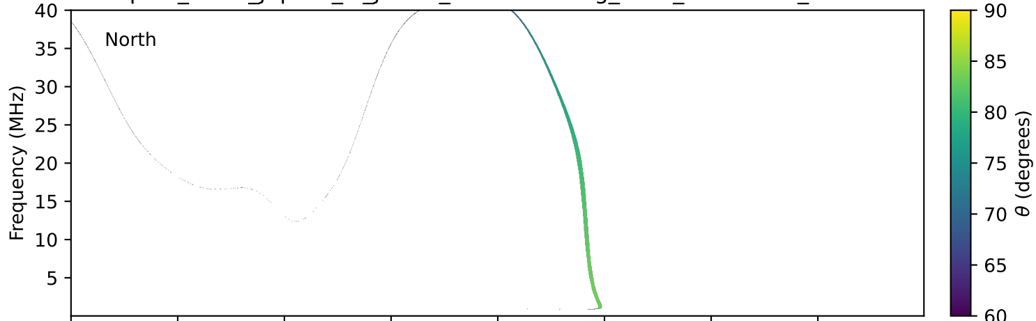
expres_earth_jupiter_io_jrm33_lossc-wid1deg_3kev_20001130_v11.cdf
