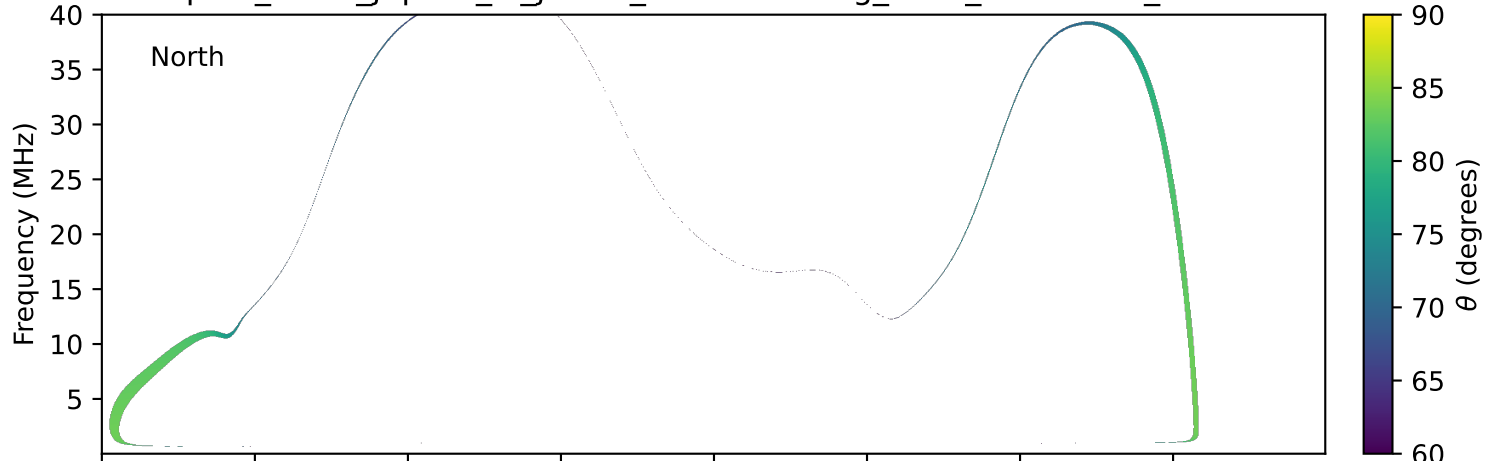
expres_earth_jupiter_io_jrm33_lossc-wid1deg_3kev_20001128_v11.cdf
