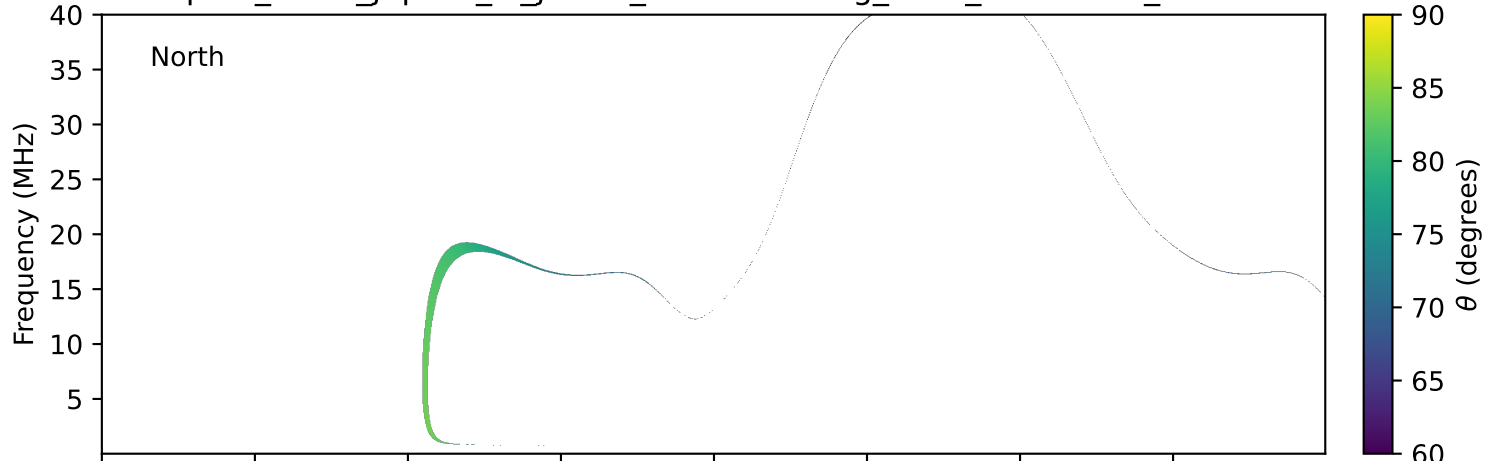
expres_earth_jupiter_io_jrm33_lossc-wid1deg_3kev_20001126_v11.cdf
