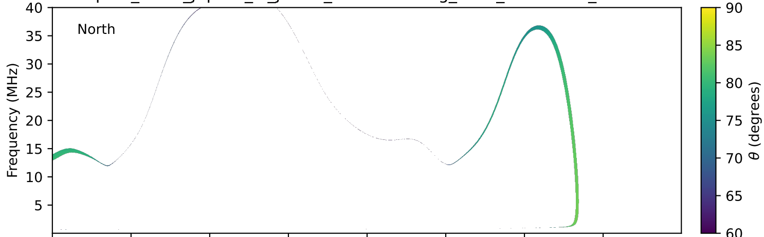
expres_earth_jupiter_io_jrm33_lossc-wid1deg_3kev_20001121_v11.cdf
