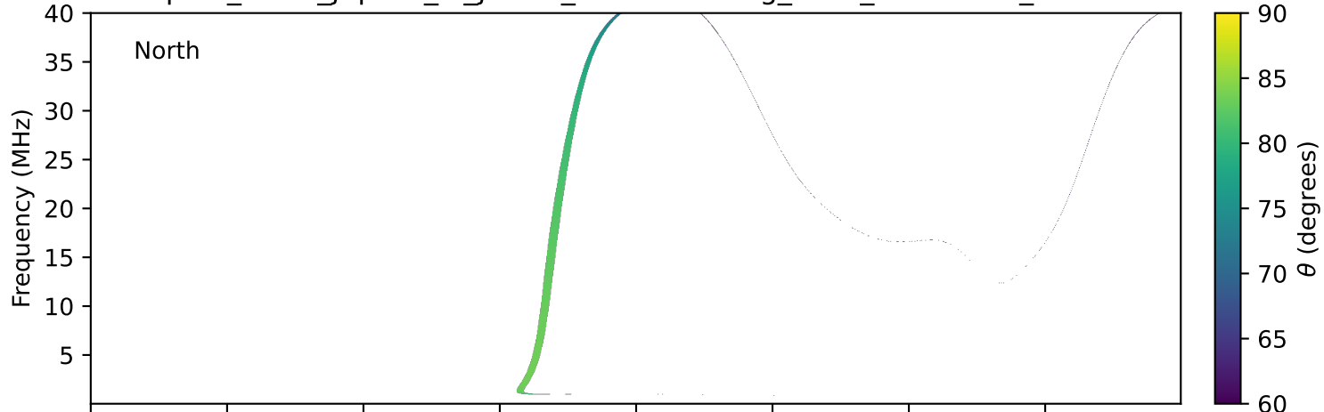
expres_earth_jupiter_io_jrm33_lossc-wid1deg_3kev_20001110_v11.cdf
