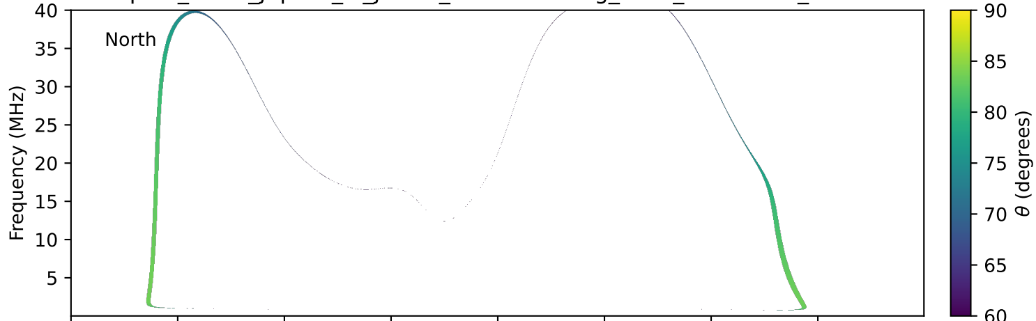
expres_earth_jupiter_io_jrm33_lossc-wid1deg_3kev_20001105_v11.cdf
