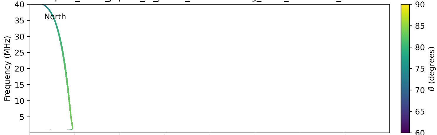
expres_earth_jupiter_io_jrm33_lossc-wid1deg_3kev_20001104_v11.cdf
