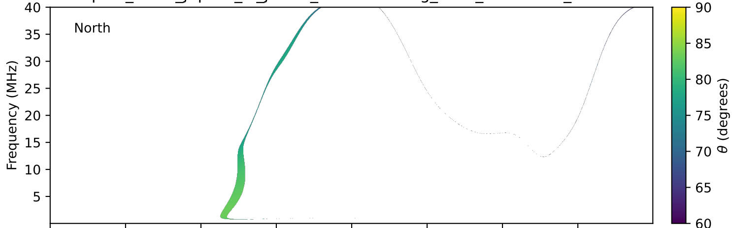
expres_earth_jupiter_io_jrm33_lossc-wid1deg_3kev_20001103_v11.cdf
