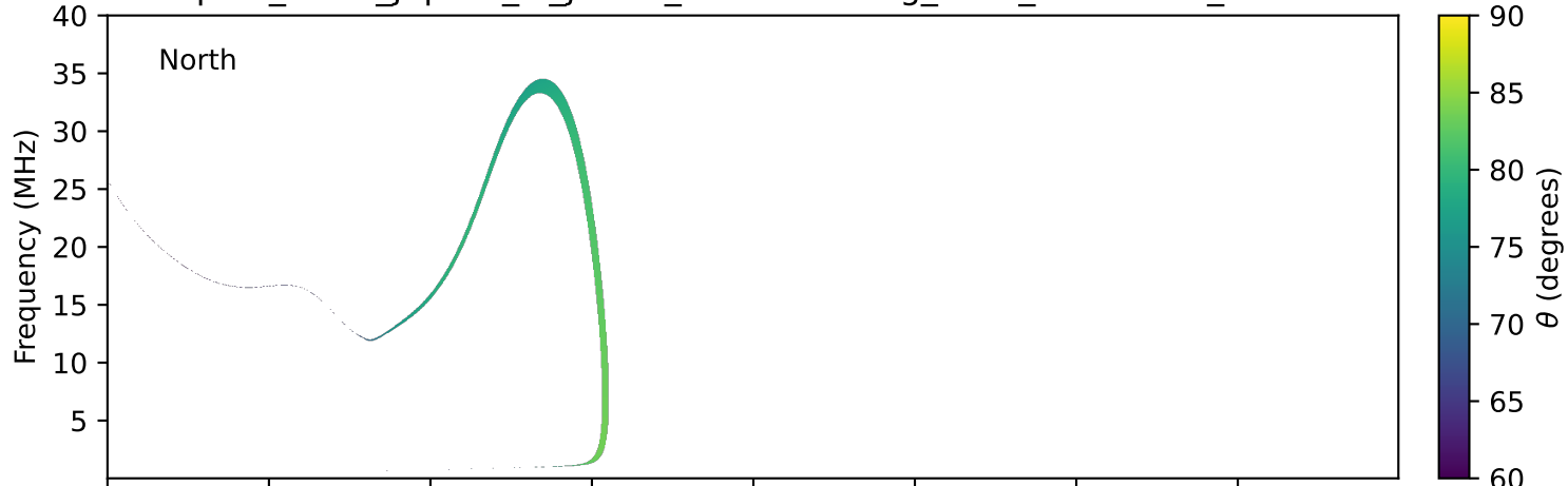
expres_earth_jupiter_io_jrm33_lossc-wid1deg_3kev_20001102_v11.cdf
