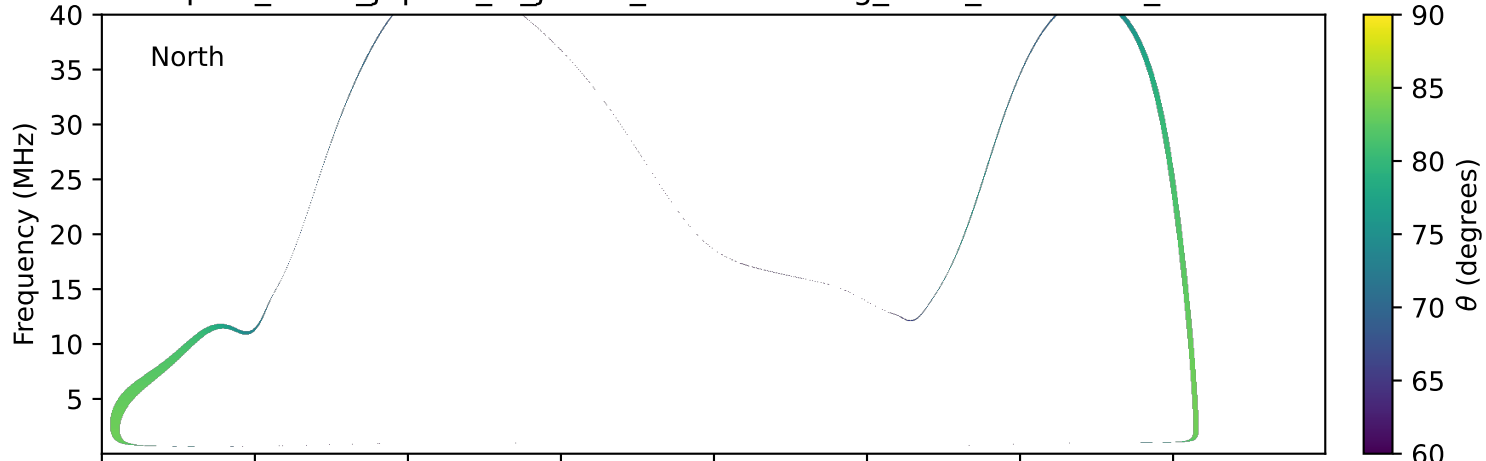
expres_earth_jupiter_io_jrm09_lossc-wid1deg_3kev_20001128_v11.cdf
