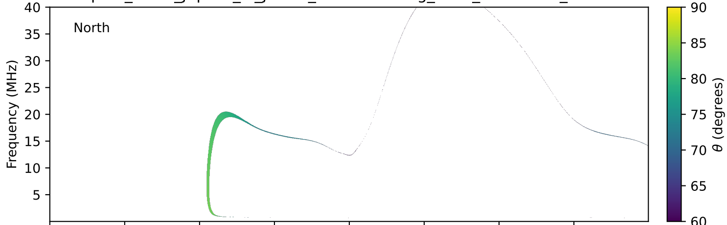
expres_earth_jupiter_io_jrm09_lossc-wid1deg_3kev_20001126_v11.cdf
