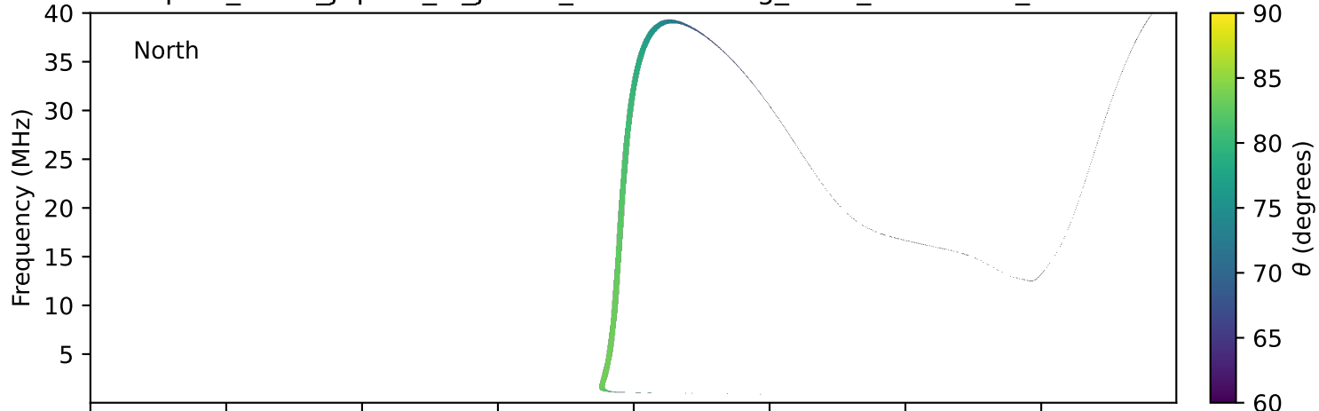
expres_earth_jupiter_io_jrm09_lossc-wid1deg_3kev_20001117_v11.cdf
