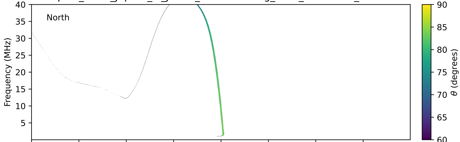
expres_earth_jupiter_io_jrm09_lossc-wid1deg_3kev_20001116_v11.cdf
