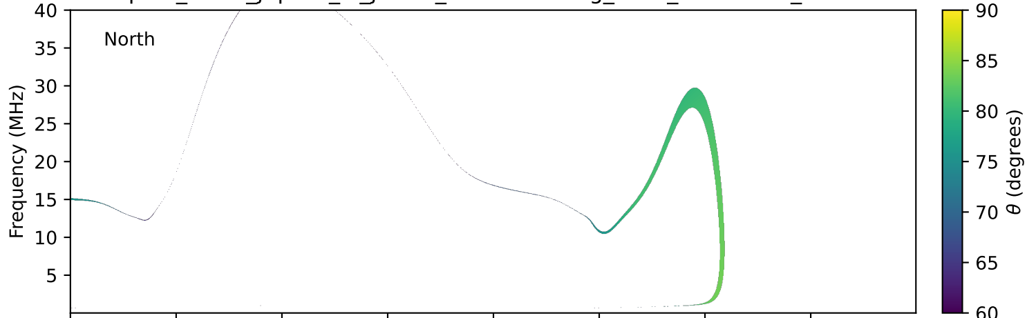
expres_earth_jupiter_io_jrm09_lossc-wid1deg_3kev_20001114_v11.cdf
