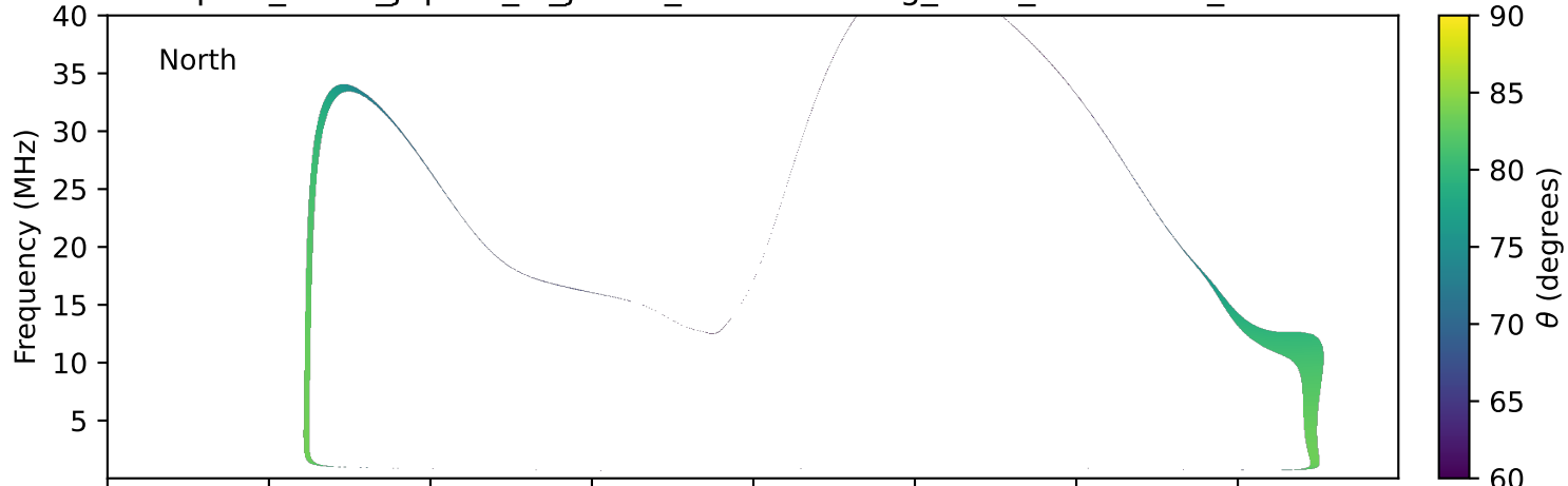
expres_earth_jupiter_io_jrm09_lossc-wid1deg_3kev_20001112_v11.cdf
