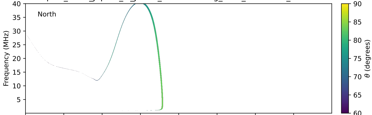
expres_earth_jupiter_io_jrm09_lossc-wid1deg_3kev_20001109_v11.cdf
