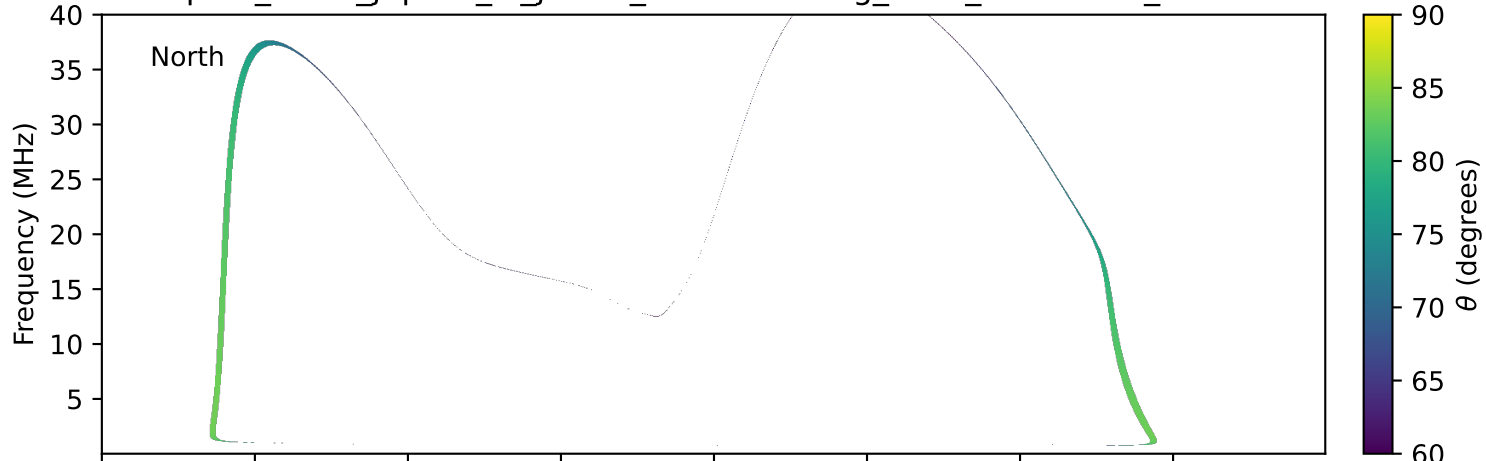
expres_earth_jupiter_io_jrm09_lossc-wid1deg_3kev_20001105_v11.cdf
