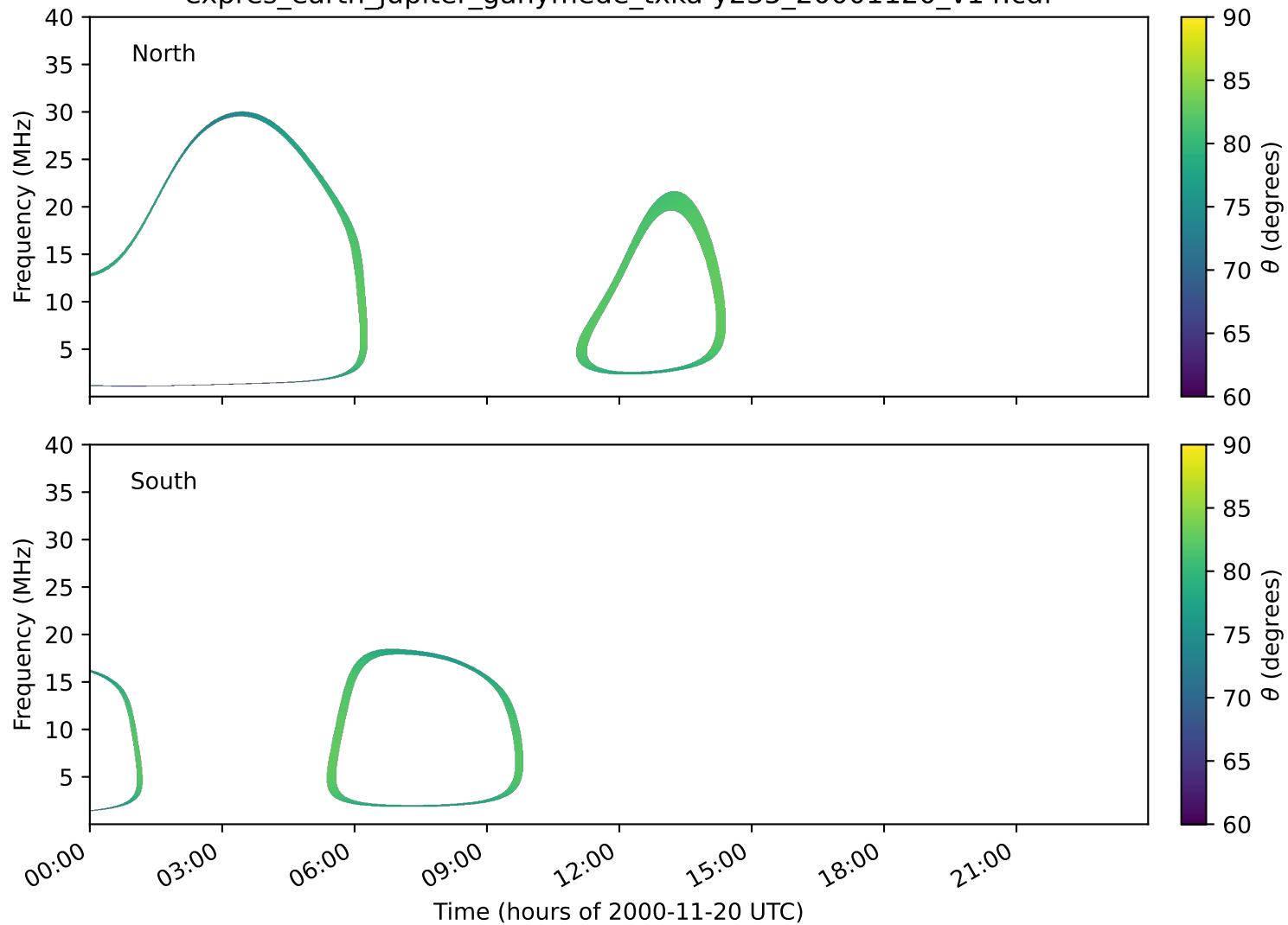
expres_earth_jupiter_ganymede_txka-y235_20001120_v14.cdf
