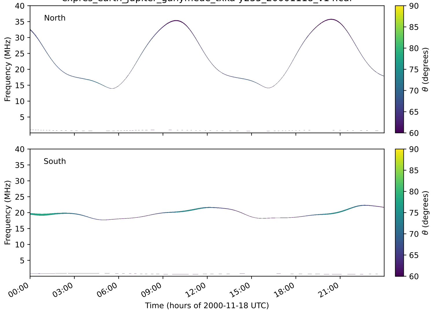
expres_earth_jupiter_ganymede_txka-y235_20001118_v14.cdf
