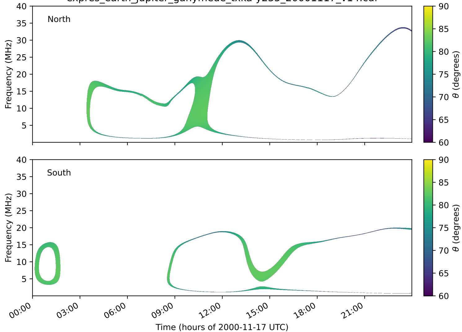
expres_earth_jupiter_ganymede_txka-y235_20001117_v14.cdf
