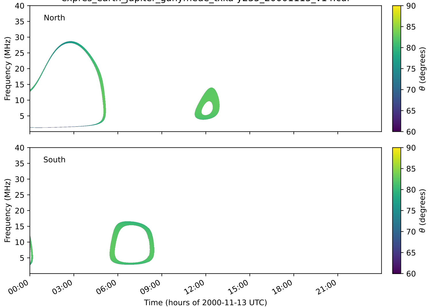
expres_earth_jupiter_ganymede_txka-y235_20001113_v14.cdf
