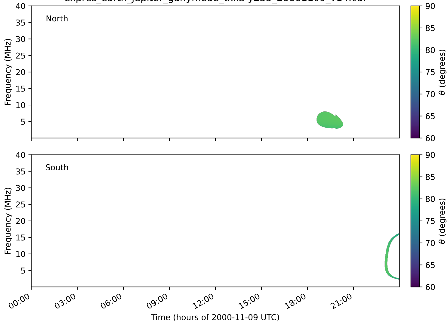
expres_earth_jupiter_ganymede_txka-y235_20001109_v14.cdf
