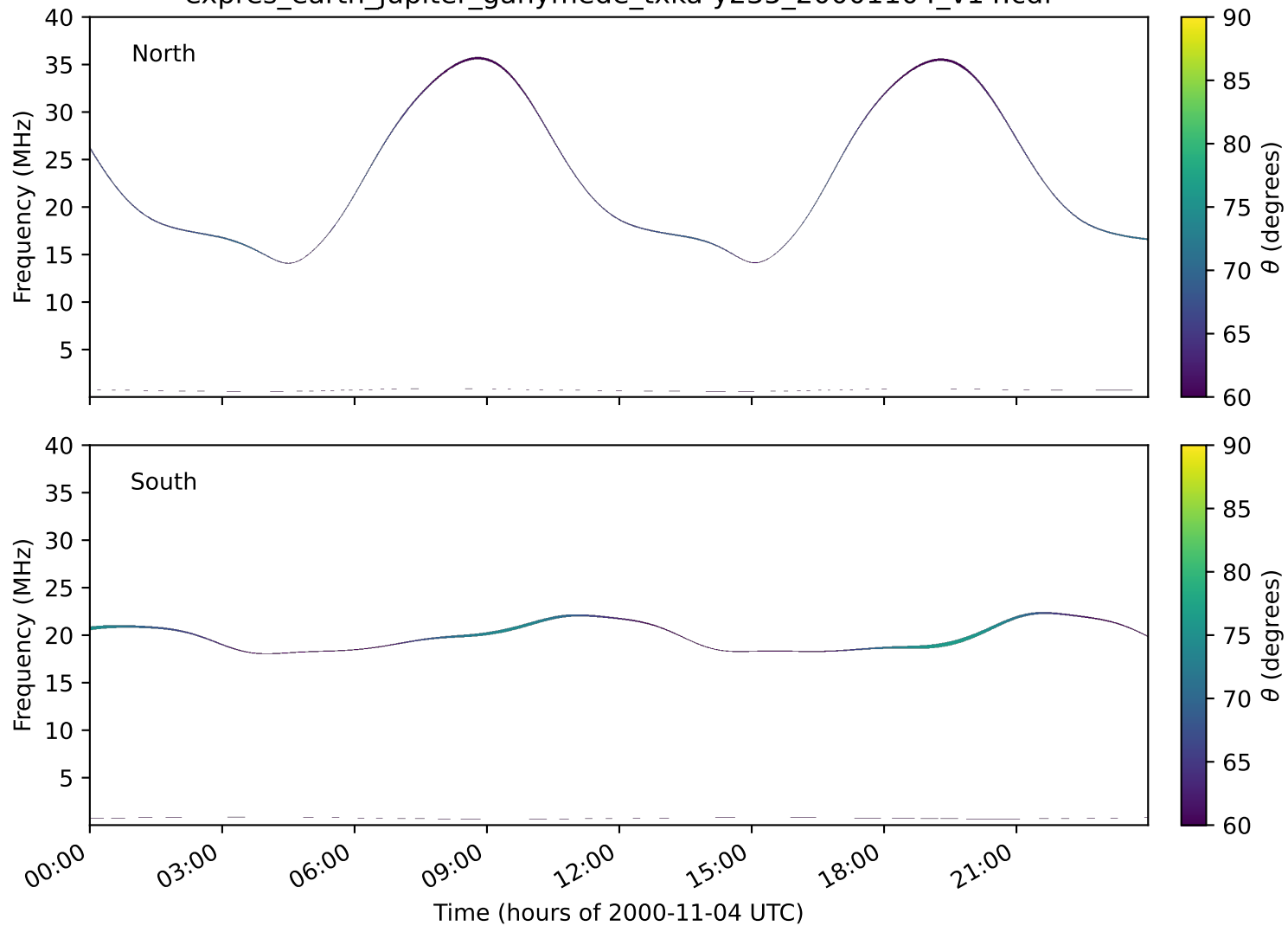
expres_earth_jupiter_ganymede_txka-y235_20001104_v14.cdf
