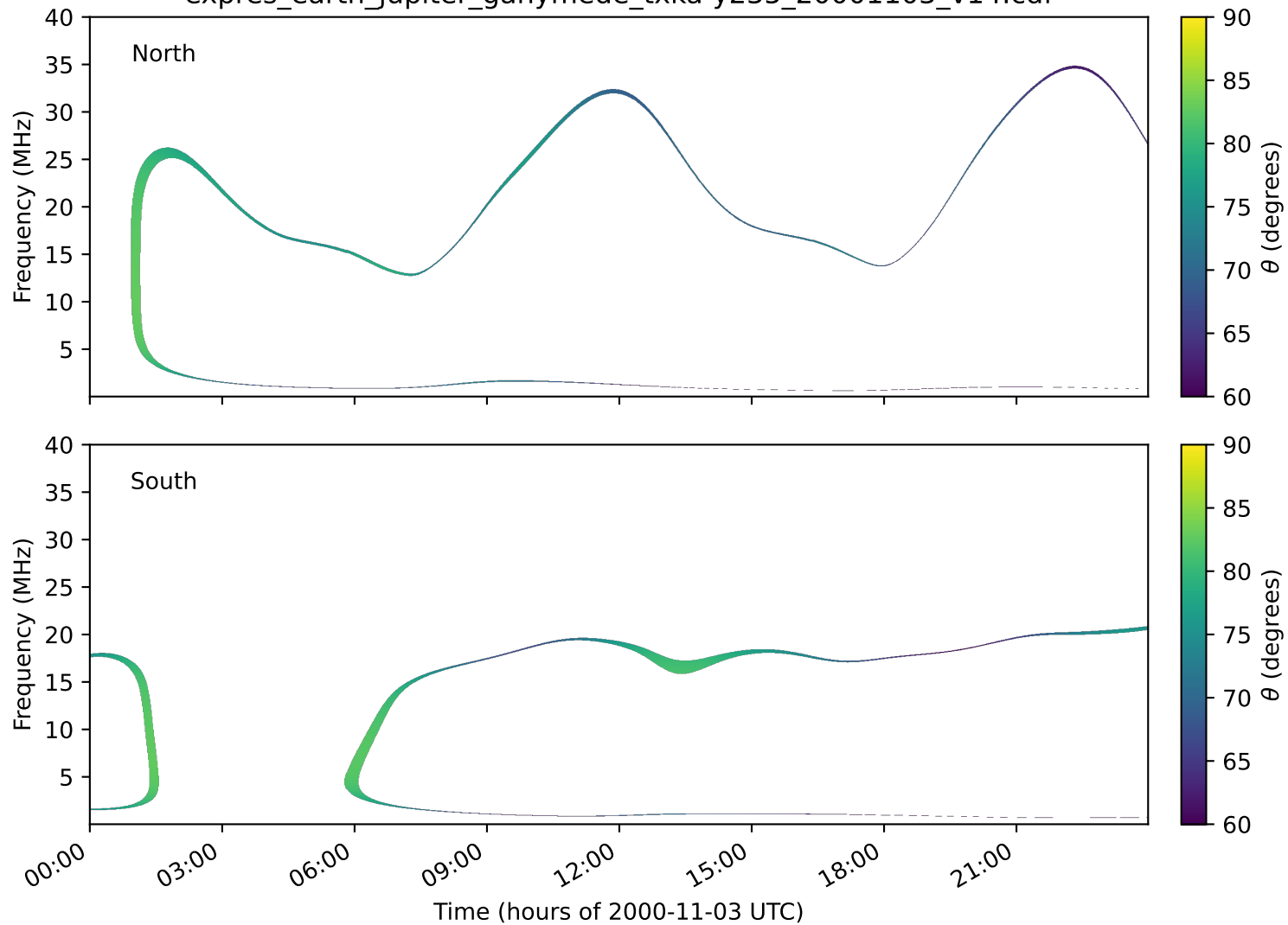
expres_earth_jupiter_ganymede_txka-y235_20001103_v14.cdf
