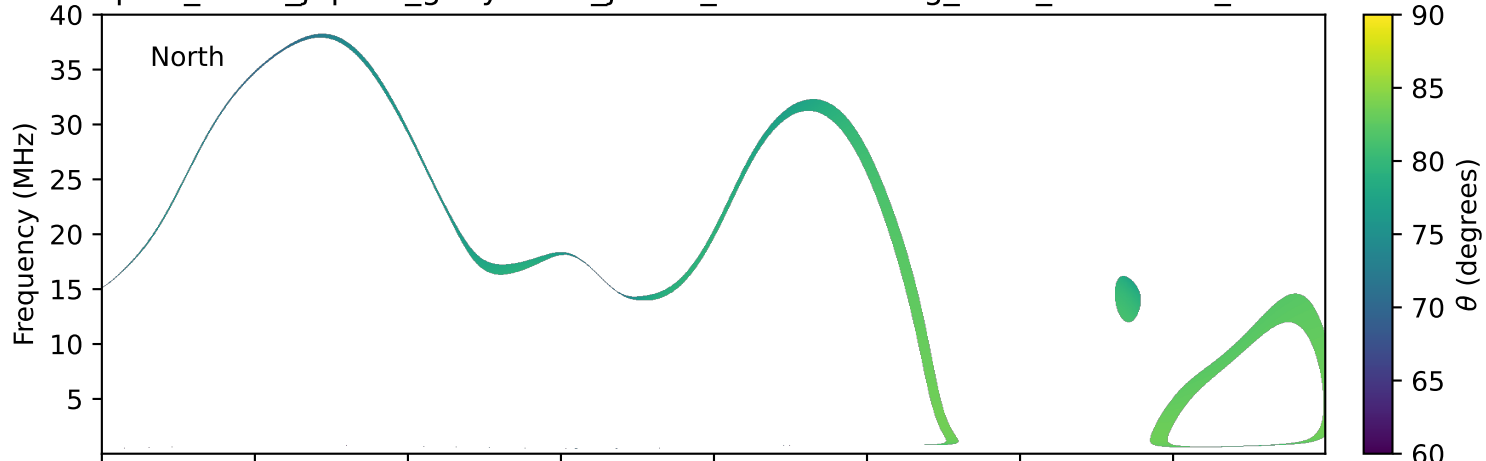
expres_earth_jupiter_ganymede_jrm33_lossc-wid1deg_3kev_20001127_v11.cdf
