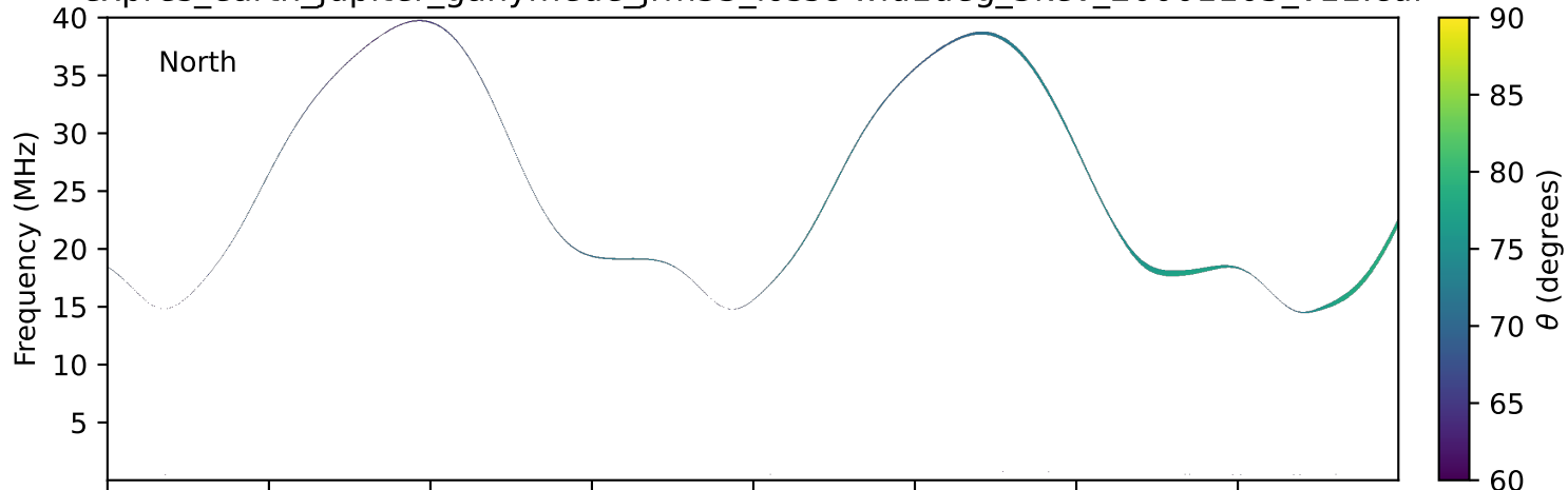
expres_earth_jupiter_ganymede_jrm33_lossc-wid1deg_3kev_20001105_v11.cdf
