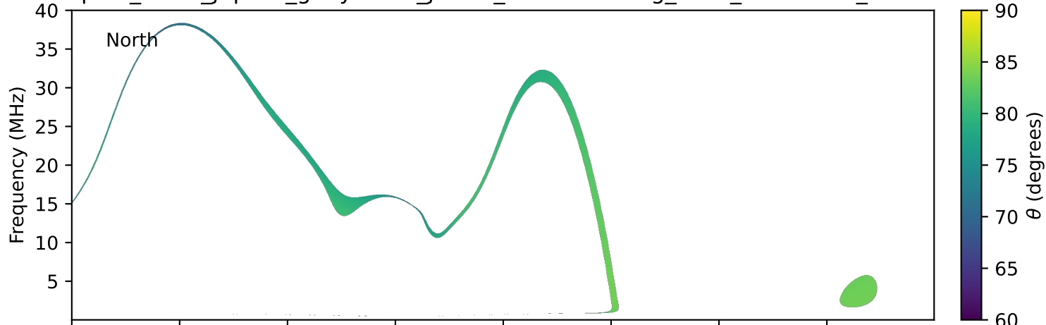
expres_earth_jupiter_ganymede_jrm09_lossc-wid1deg_3kev_20001120_v11.cdf
