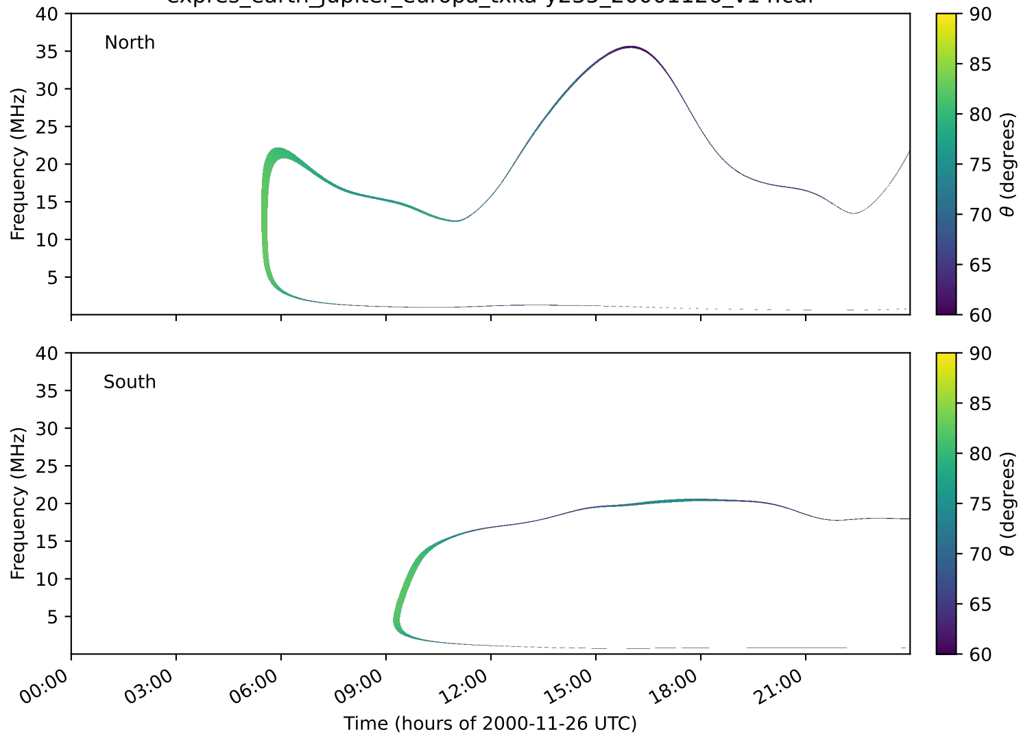
expres_earth_jupiter_europa_txka-y235_20001126_v14.cdf
