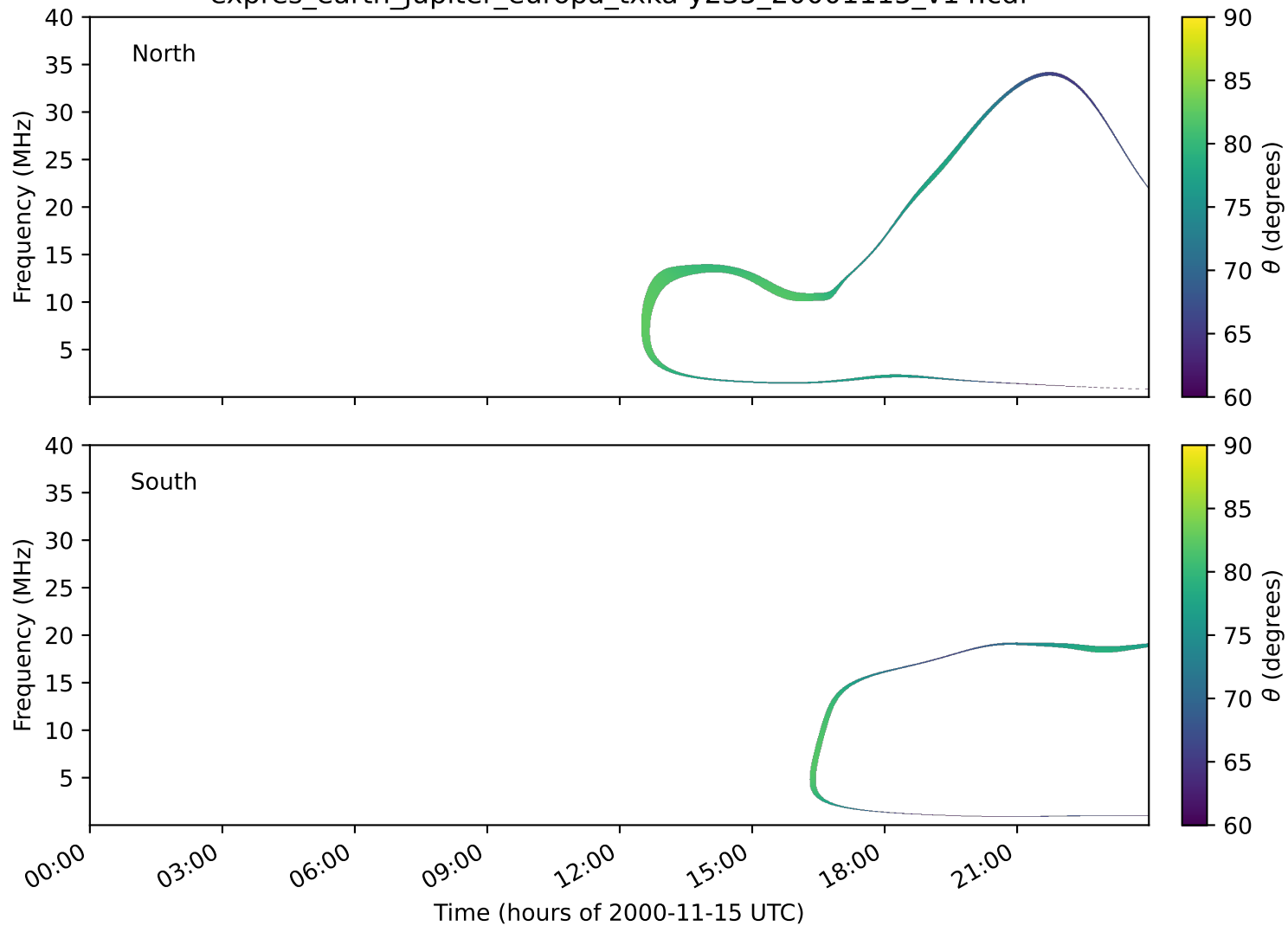
expres_earth_jupiter_europa_txka-y235_20001115_v14.cdf
