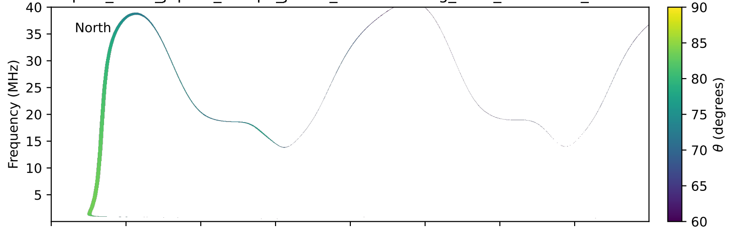
expres_earth_jupiter_europa_jrm33_lossc-wid1deg_3kev_20001105_v11.cdf
