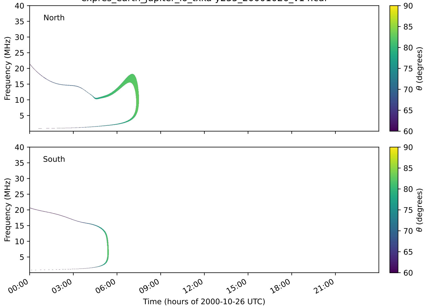
expres_earth_jupiter_io_txka-y235_20001026_v14.cdf
