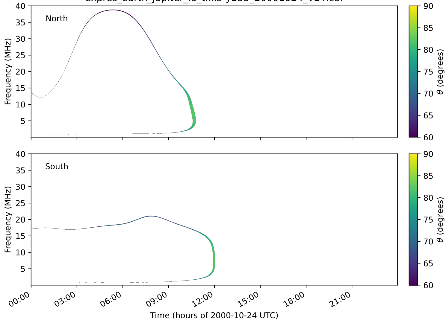
expres_earth_jupiter_io_txka-y235_20001024_v14.cdf
