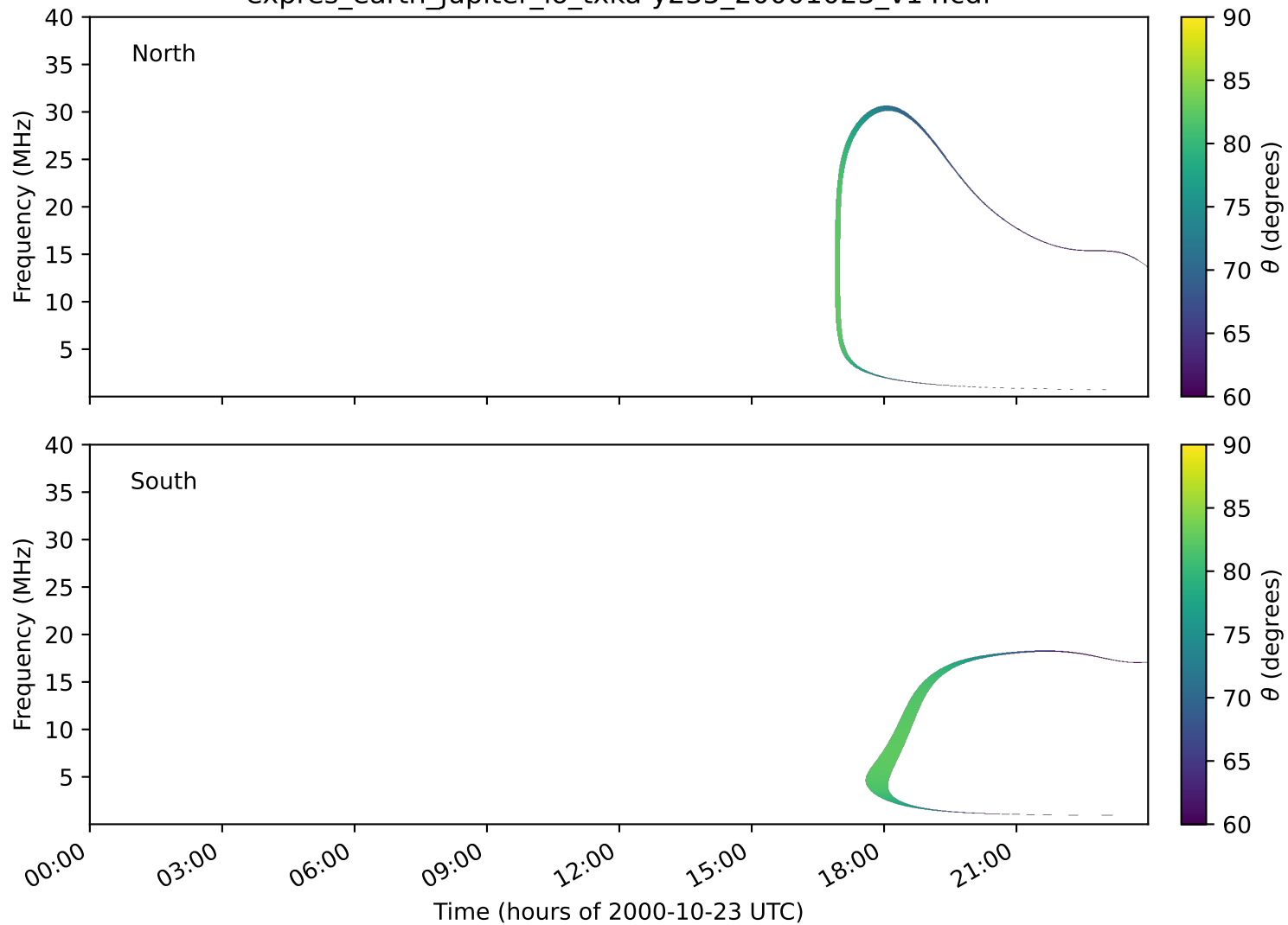
expres_earth_jupiter_io_txka-y235_20001023_v14.cdf
