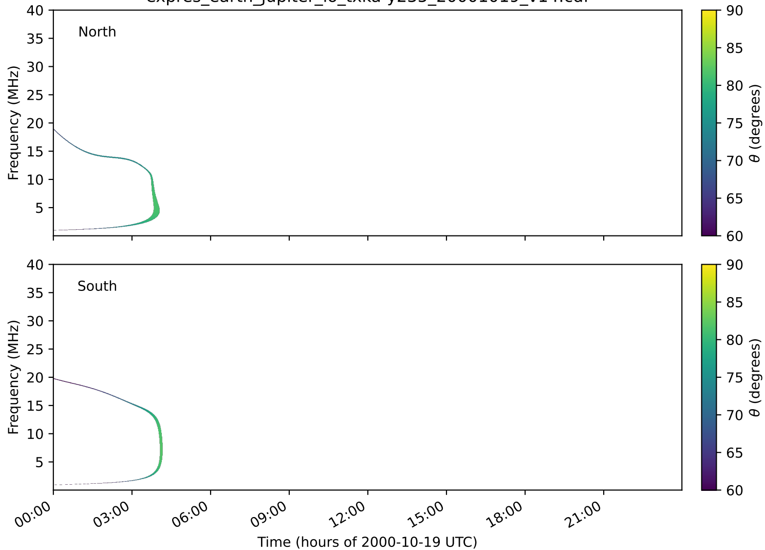
expres_earth_jupiter_io_txka-y235_20001019_v14.cdf
