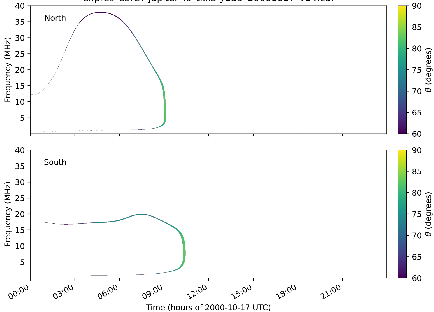
expres_earth_jupiter_io_txka-y235_20001017_v14.cdf
